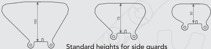
Standard heights for side guards
